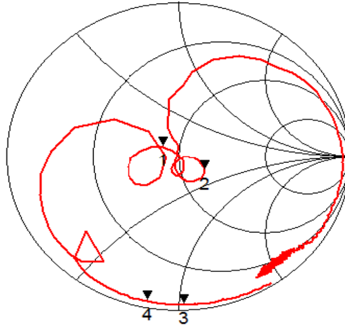
Smith Chart S22
