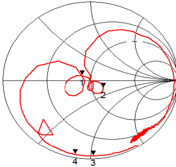
Smith Chart S11
